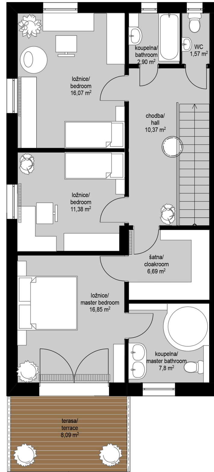
PATRO/FIRST FLOOR
